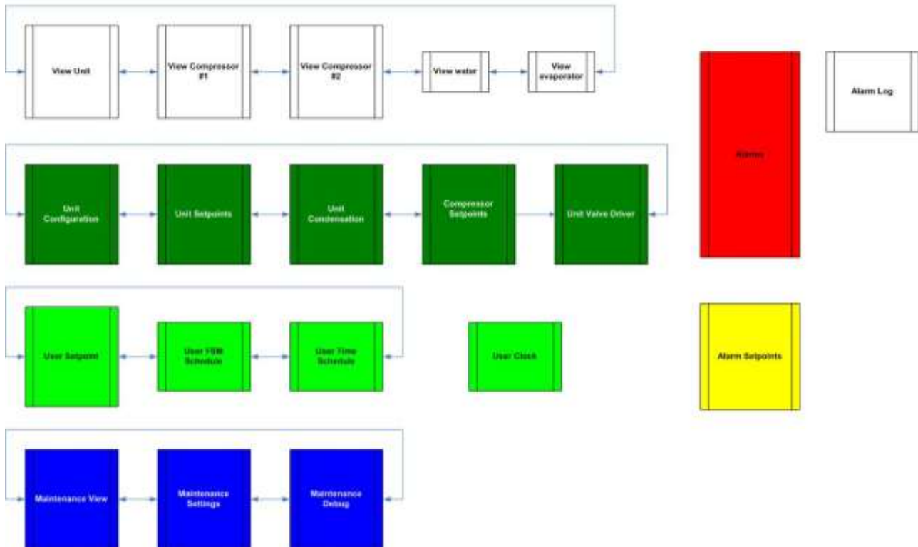
Fig 25 – HMI structure
