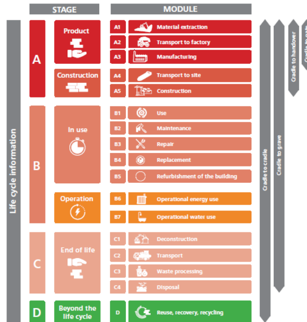
Figure 1. Graphical representation of life cycle assessment
