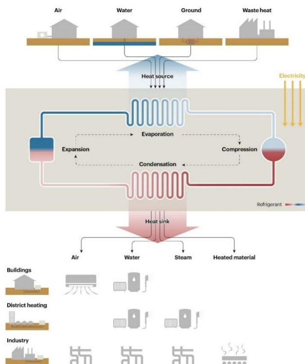
FIGURE 0.1 HOW A HEAT PUMP WORKS SOURCE: IEA THE FUTURE OF HEAT PUMPS (2022)
