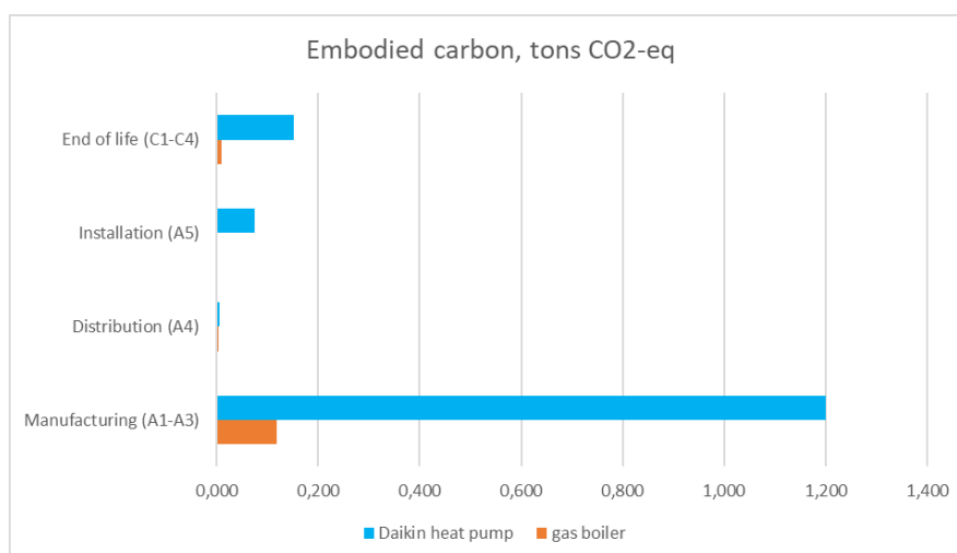
Figure 5. Comparison of embodied carbon for Daikin heat pump and gas boiler
