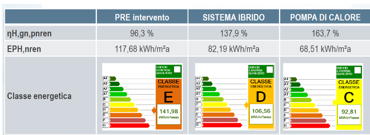
FIGURE 0.8 SOURCES: EDILCLIMA SIMULATIONS
