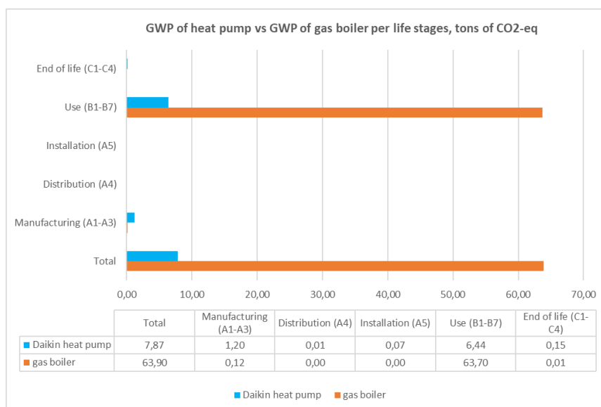
Figure 4. Comparison of full LCA for Daikin heat pump and gas boiler
