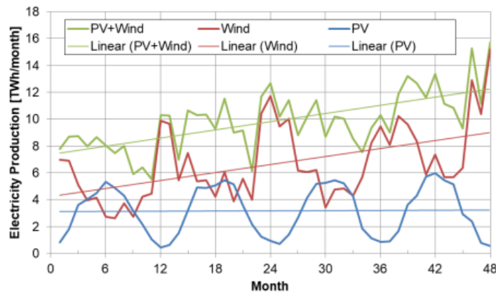
Figure 25: Monthly production of PV and wind power for 2014 - 2017 [ISE4].
