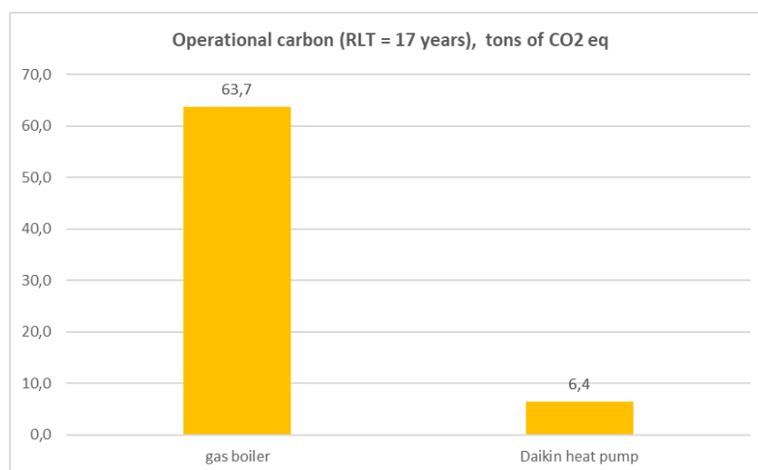
Figure 6. Comparison of operational carbon for Daikin heat pump and gas boiler
