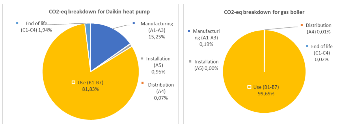
Figure 3. Breakdown of CO 2 -eq per life stages for heat pump and gas boiler, %
